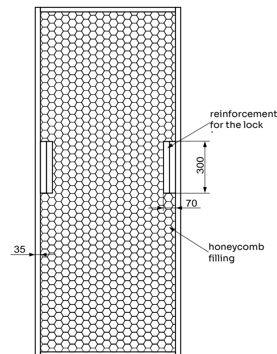
Panel door leaves construction
