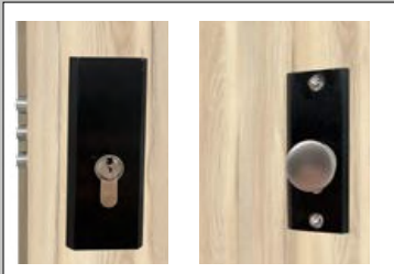
BOTTOM LOCK
