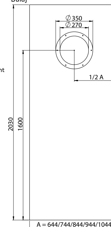
Rebated door leaf Bulaj
