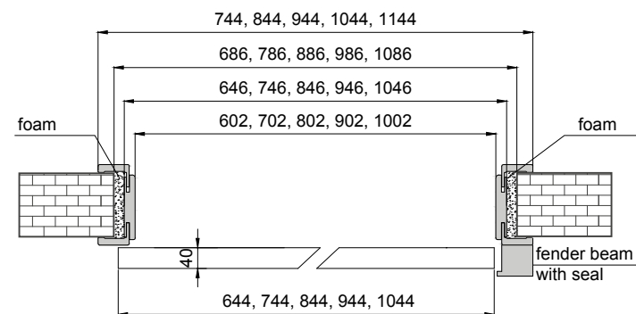
FENDER BEAM
