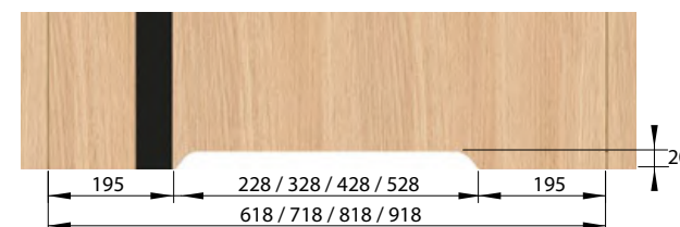
VENTILATION UNDERCUT OF MODERNO, LAMELO, MAGNETIC L, INTARSIA 40
