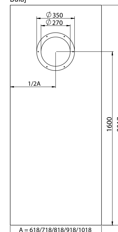
Non-rebated door leaf Bulaj
