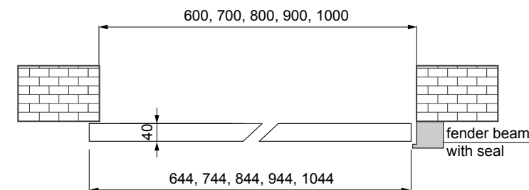
WITHOUT CASING
