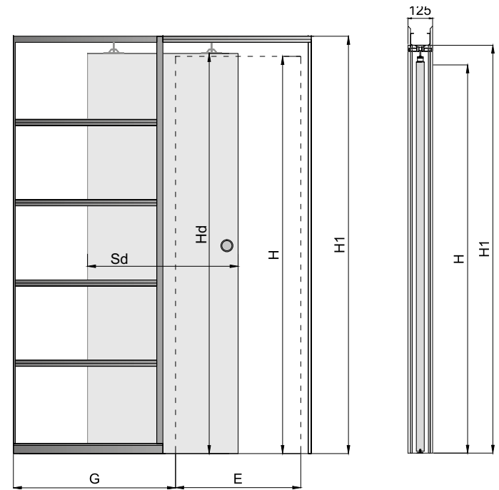
SINGLE CASSETTE G/K door leaf
