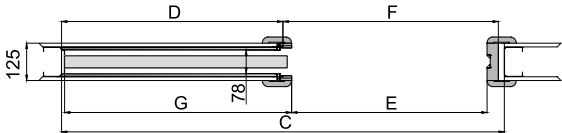
Cassette G/K – single aluminium sliding system Door closer
