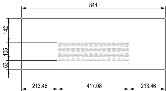
Protective panel with ventilation – dimensions for a door leaf with a width of "80", rebated door leaf, obverse side
