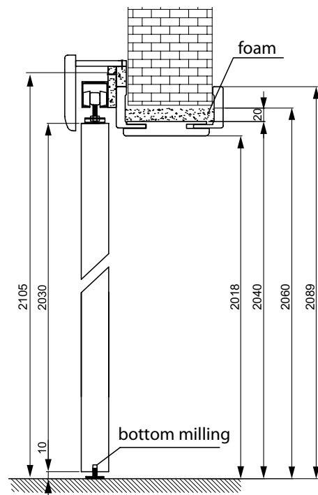
WITH CASING - TUNNEL
