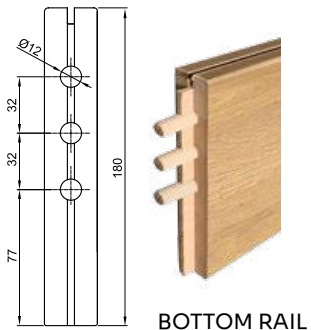
BOTTOM RAIL
