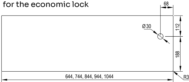
Central protective panel with holes for the economic lock
